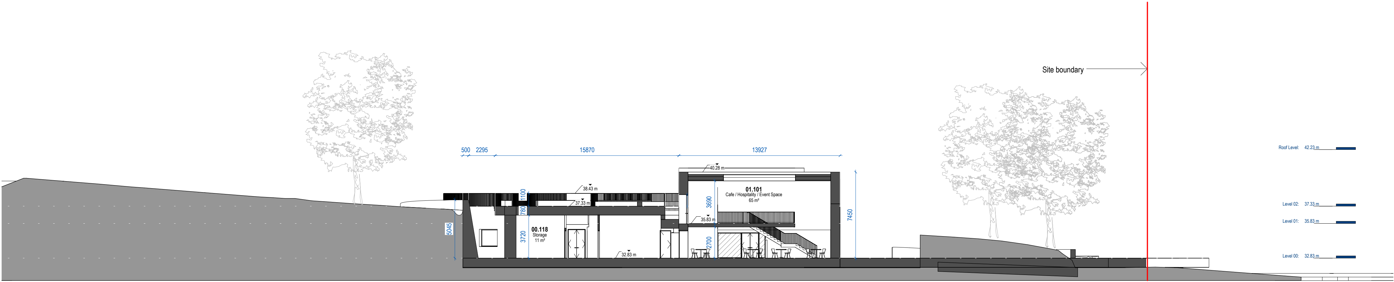
1 Proposed Section CC Scale - 1:200
